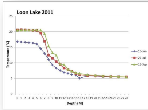
Figure 2. nbsp; Loon Lake Water Column Temperature profiles
