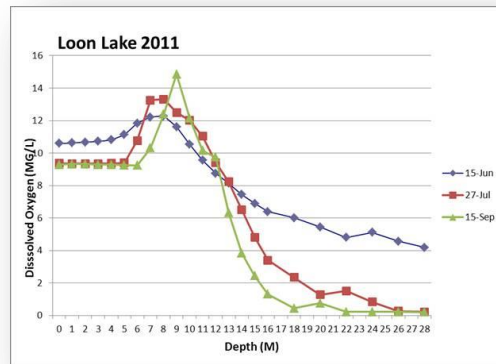
Figure 3: Loon Lake Dissolved Oxygen Profiles – Note: Dissolved Oxygen is shown in milligrams per liter (mg/L). A milligram is one one thousandths of a gram.
